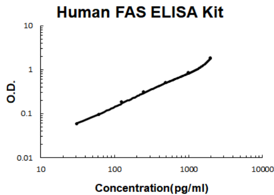
Human FAS PicoKine ELISA Kit standard curve
