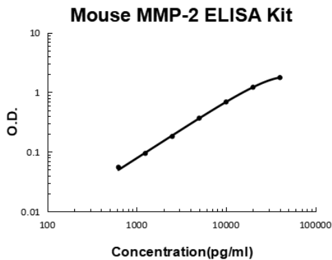
Mouse MMP-2 PicoKine ELISA Kit standard curve
