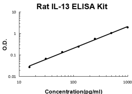
Rat IL-13 PicoKine ELISA Kit standard curve
