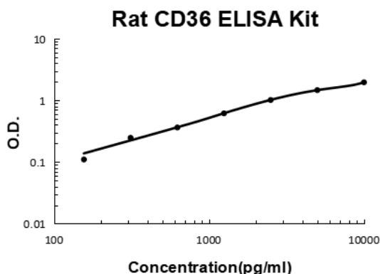
Rat CD36/SR-B3 PicoKine ELISA Kit standard curve
