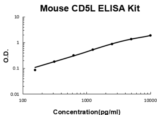
Mouse CD5L PicoKine ELISA Kit standard curve
