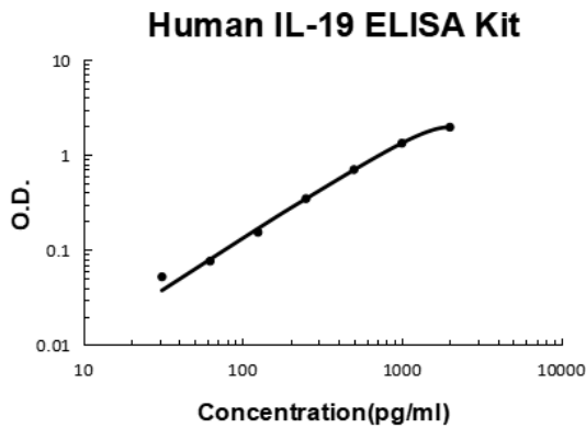
Human IL-19 PicoKine ELISA Kit standard curve
