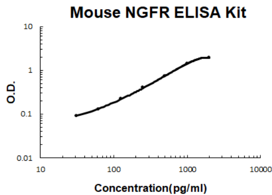
Mouse NGFR PicoKine ELISA Kit standard curve
