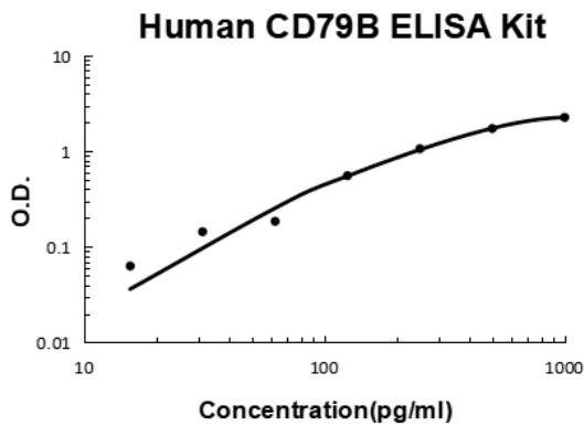
Human CD79B PicoKine ELISA Kit standard curve
