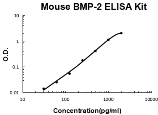
Mouse BMP-2 PicoKine ELISA Kit standard curve
