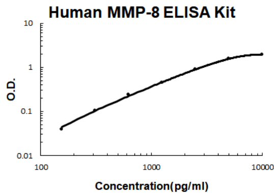
Human MMP-8 PicoKine ELISA Kit standard curve
