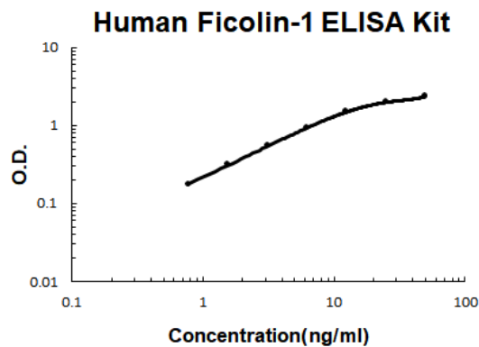
Human Ficolin-1 PicoKine ELISA Kit standard curve
