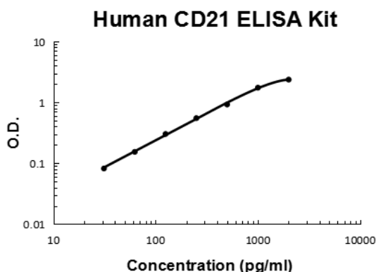
Human CD21 PicoKine ELISA Kit standard curve
