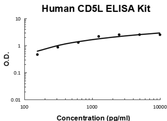
Human CD5L PicoKine ELISA Kit standard curve
