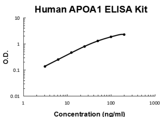
Human APOA1 PicoKine ELISA Kit standard curve
