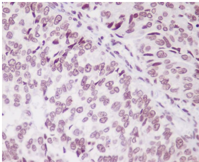
Immunohistochemical analysis of paraffin-embedded human bladder cancer, using PARK7 Antibody.
