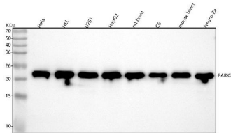
Figure 1. Western blot analysis of PARK7 using anti-PARK7 antibody (M00757).
