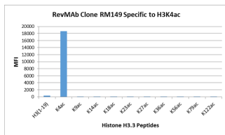
Figure 2. Specificity Test result RM149 specifically reacts to Histone H3 acetylated at Lysine 4 (K4ac). No cross reactivity with non-modified Lysine 4, acetylated Lysine 9 (K9ac), Lysine 14 (K14ac), Lysine 18 (K18ac), Lysine 23 (K23ac), Lysine 27 (K27ac), Lysine 36 (K36ac), Lysine 56 (K56ac), lysine 79 (K79ac), or Lysine 122 (K122) in histone H3.
