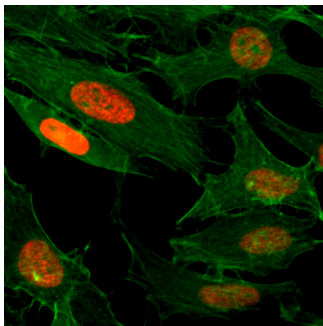
Figure 3. ICC result Immunocytochemistry of HeLa cells treated with sodium butyrate, using Acetyl-Histone H3 (Lys4) Rabbit mAb RM149 (red). Actin filaments have been labeled with fluorescein phalloidin (green).
