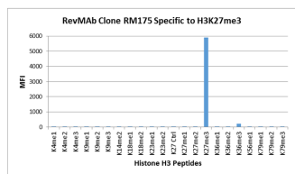
Figure 2. Specificity Test result RM175 specifically reacts to Histone H3 trimethylated at Lysine 27 (K27me3). No cross reactivity with non-modified Lysine 27 (K27 Ctrl), monomethylated Lysine 27 (K27me1) or dimethylated Lysine 27 (K27me2), or other methylations in Histone H3.
