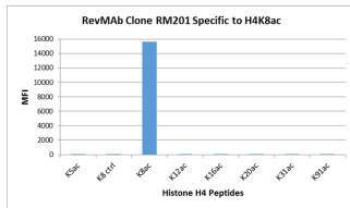
Figure 2. Specificity Test result RM201 specifically reacts to Histone H4 acetylated at Lysine 8 (K8ac). No cross reactivity with unmodified Lysine 8 (K8 ctrl), acetylated Lysine 5 (K5ac), Lysine 12 (K12ac), Lysine 16 (K16ac), Lysine 20 (K20ac), Lysine 31 (K31ac), or Lysine 91 (K91) in Histone H4.
