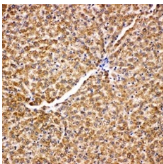
Figure 3. IHC analysis of Grp75 using anti-Grp75 antibody (PA1789).
