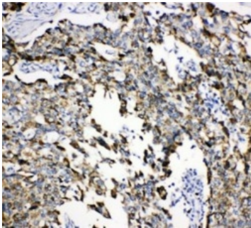
Figure 2. IHC analysis of Grp75 using anti-Grp75 antibody (PA1789).
