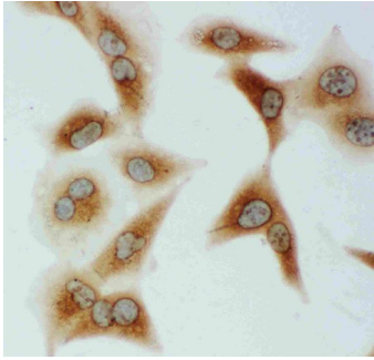
Figure 4. ICC analysis of Grp75 using anti-Grp75 antibody (PA1789).
