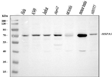
Figure 1. Western blot analysis of Grp75 using anti-Grp75 antibody (PA1789).
