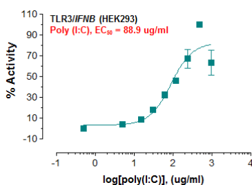
Fig-1: Induction of TLR3 activity by poly(I:C) in TLR3/IFNB HEK293 cells.
