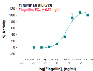
Fig-1: Induction of TLR5 activity by Flagellin in TLR5/NF- \kappa B HEK293 cells.
