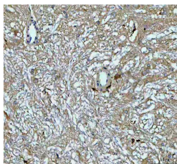
Figure 2. IHC analysis of GH1 using antiGH1 antibody (RP1007).
