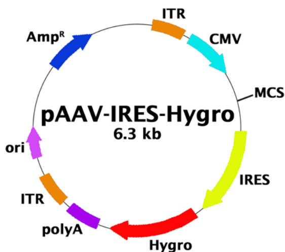
Figure 3: pAAV-IRES-Hygro Expression Vector (see Appendix for more detail).
