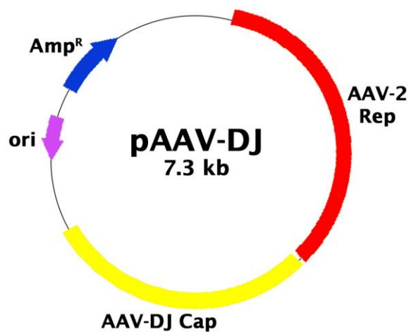
Figure 4. pAAV-DJ Vector
