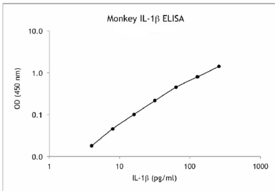
Example of a representative Monkey IL-1 \beta standard curve using a 4-parameter logistic fit.
