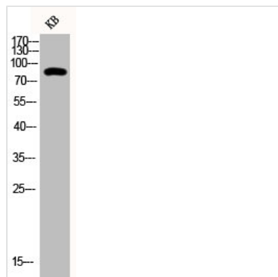
Western Blot analysis of KB cells using Phospho-Stat3 (Y705) Polyclonal Antibody
