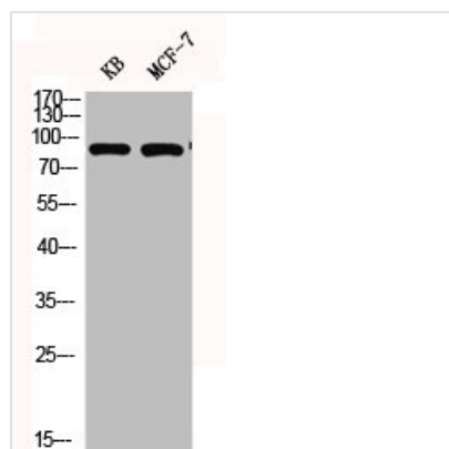
Western Blot analysis of KB MCF7 cells using Phospho-Stat3 (Y705) Polyclonal Antibody
