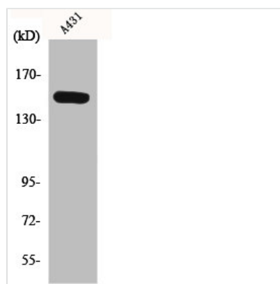
Western Blot analysis of A431 cells using Phospho-PLC \beta 3 (S1105) Polyclonal Antibody
