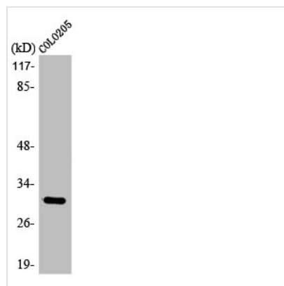
Western Blot analysis of HuvEc cells using ABHD11 Polyclonal Antibody
