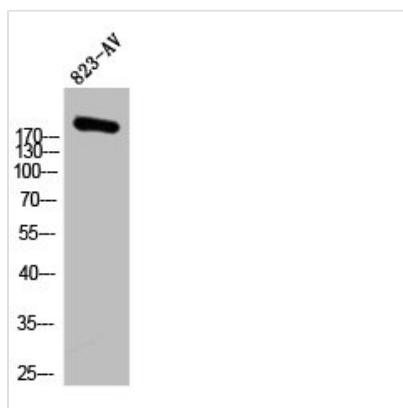
Western Blot analysis of 823-AV cells using ACC \alpha Polyclonal Antibody
