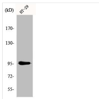
Western Blot analysis of HT29 cells using Dnmt3b Polyclonal Antibody
