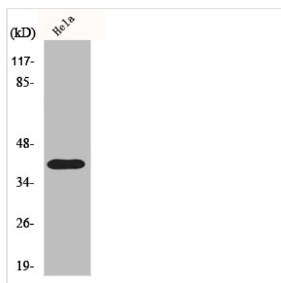
Western Blot analysis of HuvEc cells using P2RY8 Polyclonal Antibody
