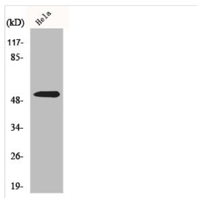
Western Blot analysis of HuvEc cells using Parkin Polyclonal Antibody
