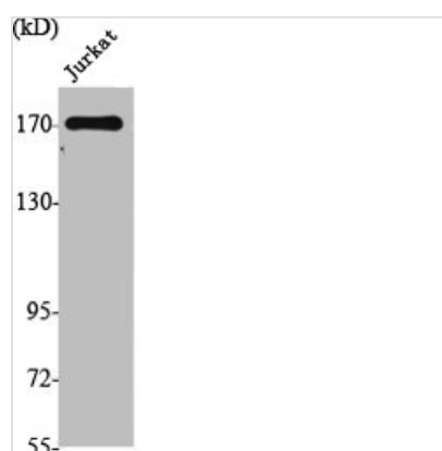
Western Blot analysis of Jurkat cells using Topo IIα Polyclonal Antibody
