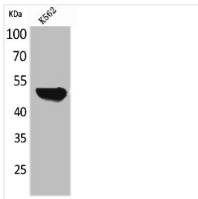
Western Blot analysis of K562 cells using Protein C Polyclonal Antibody
