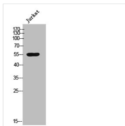
Western Blot analysis of Jurkat cells using Csk Polyclonal Antibody
