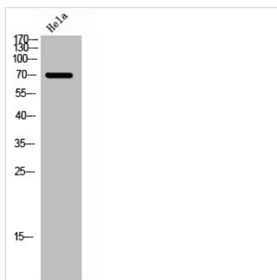
Western Blot analysis of HELA cells using Phospho-FoxO1 (S256) Polyclonal Antibody
