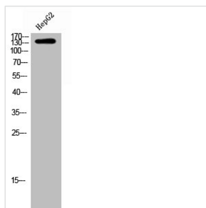
Western Blot analysis of HEPG2 cells using Flt3 Polyclonal Antibody
