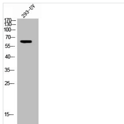
Western Blot analysis of 293 cells using Phospho-TH (S62) Polyclonal Antibody
