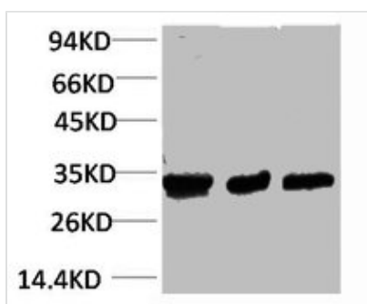
Western blot analysis of 1) Human Brain Tissue, 2) Mouse Brain Tissue, 3) Rat Brain Tissue using CACNG3 Polyclonal Antibody.
