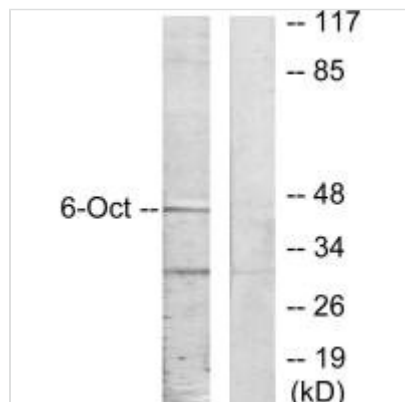
Western blot analysis of extracts from A549 cells, using OCT6 antibody.
