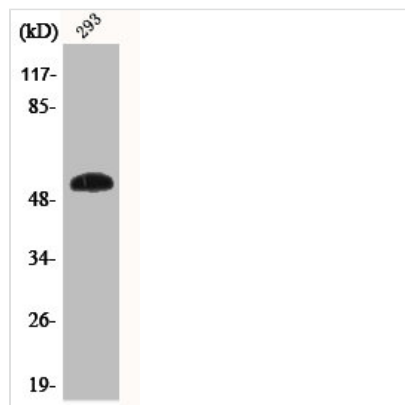
Western Blot analysis of 293 cells using Phospho-p53 (S46) Polyclonal Antibody
