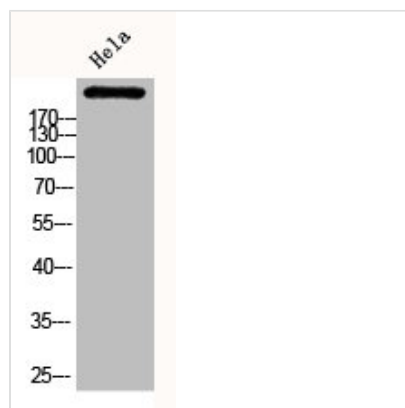
Western Blot analysis of HELA cells using Phospho-ACC \alpha (S80) Polyclonal Antibody
