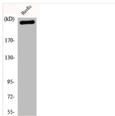
Western Blot analysis of HuvEc cells using Filamin 1 Polyclonal Antibody
