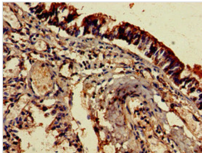
Immunohistochemistry of paraffin-embedded human lung tissue using CSB-PA007404LA01HU at dilution of 1:100
