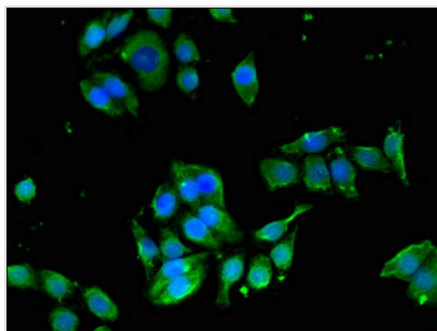
Immunofluorescent analysis of PC-3 cells using CSB-PA007404LA01HU at dilution of 1:100 and Alexa Fluor 488-conjugated AffiniPure Goat Anti-Rabbit IgG(H+L)
