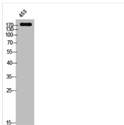
Western Blot analysis of 453 cells using Phospho-EGFR (Y1172) Polyclonal Antibody
