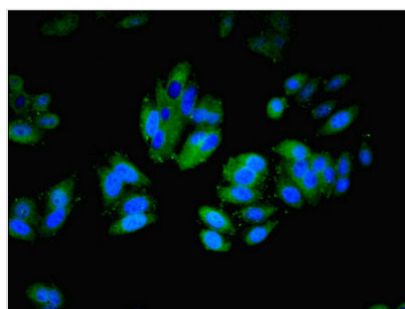
Immunofluorescent analysis of HepG2 cells using CSB-PA011875LA01HU at dilution of 1:100 and Alexa Fluor 488-conjugated AffiniPure Goat Anti-Rabbit IgG(H+L)
