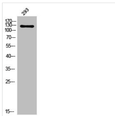
Western Blot analysis of 293 cells using USP40 Polyclonal Antibody
