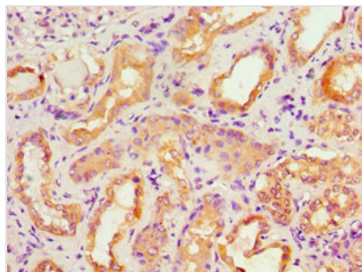
Immunohistochemistry of paraffin-embedded human kidney tissue using CSB-PA878955ESR1HU at dilution of 1:100
