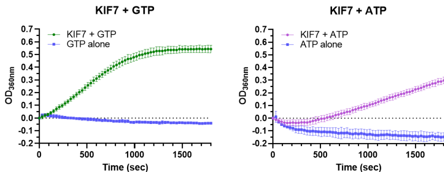
Figure 2. CS-KF51 microtubule-activated ATPase/GTPase activity using the Kinesin ELIPA Assay Kit (Cat. # BK060). KIF7 GTP or ATPase activity was assayed and data averaged with nucleotide (n=4) or control reactions with no motor (n=2) according to the method described.
