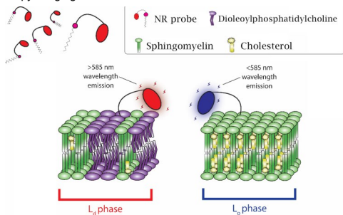
Figure 1. Diagram of NR12A's lipid order-dependent emission.
