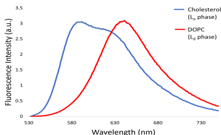
Figure 3. Fluorescence spectra of NR12A in L_0 (Cholesterol) and L_d (DOPC) phases.
